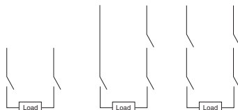
2 poles in series 3 poles in series 4 poles in series
