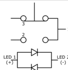
SPDT SCHEMATIC ILLUMINATED
