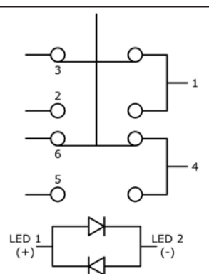
DPDT SCHEMATIC ILLUMINATED
