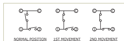
SCHEMATIC
