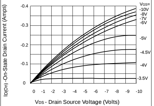
Saturation Characteristics
