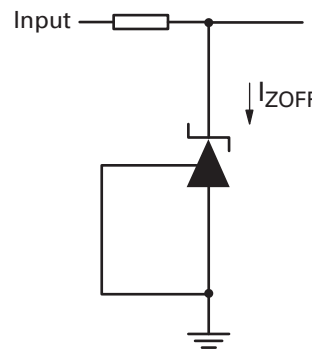
Fig 3 - Test circuit for for O state current †
