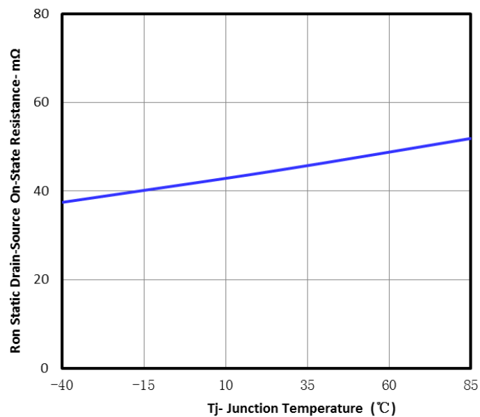
Figure 8. MOSFET r_{DS(on)} Vs. Junction Temperature
