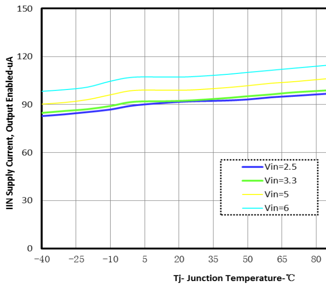
Figure 6. IIN – Supply Current, Output Enabled – μA
