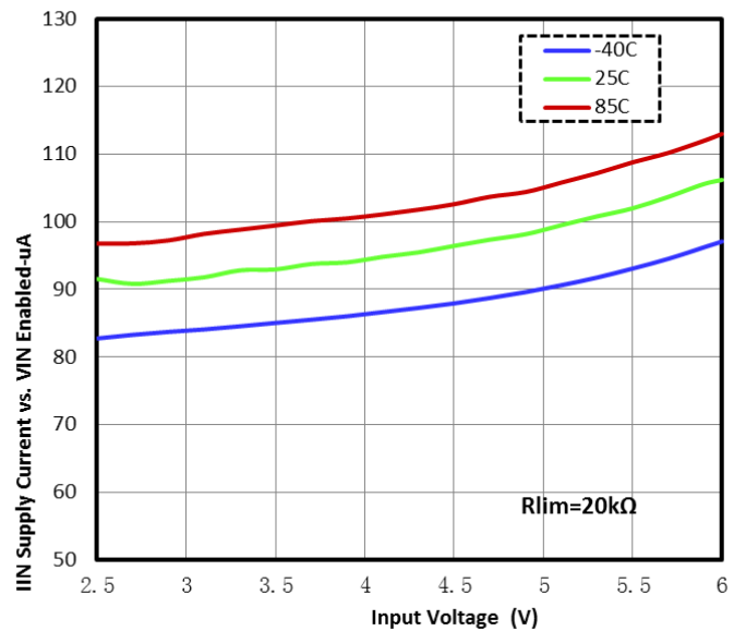
Figure 7. IIN – Supply Current, Output Enabled – μA
