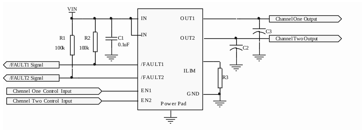
Figure3. Typical Characteristics Reference Schematic
