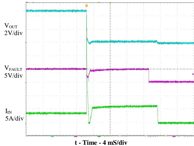
Figure 6 Full-Load to Short-Circuit Transient Response
