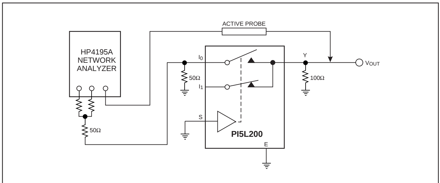
Figure 5. Off Isolation
