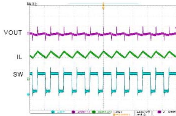
8. Switching Waveform
