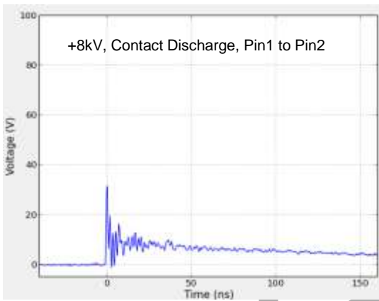
Figure 5. ESD response ESD response to IEC 61000-4-2
