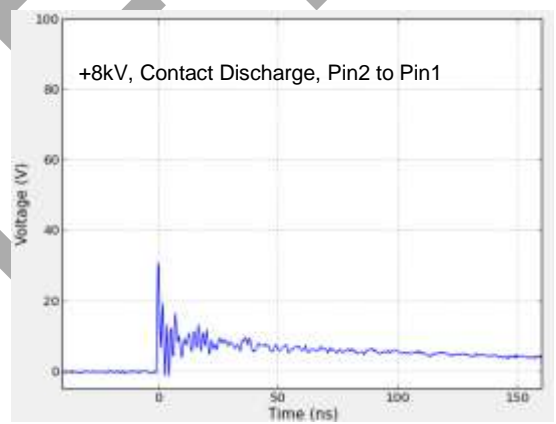
Figure 6. ESD response ESD response to IEC 61000-4-2
