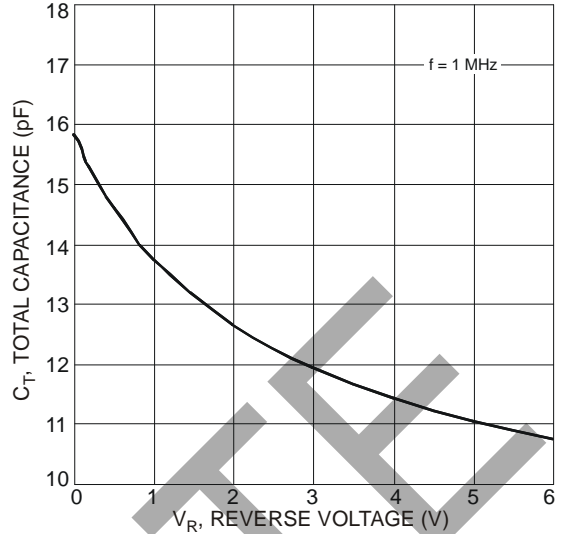
Figure 2 Typical Total Capacitance vs. Reverse Voltage
