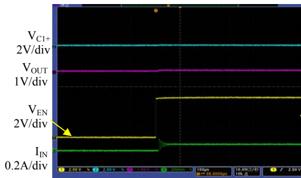
Time (100μs/div)
