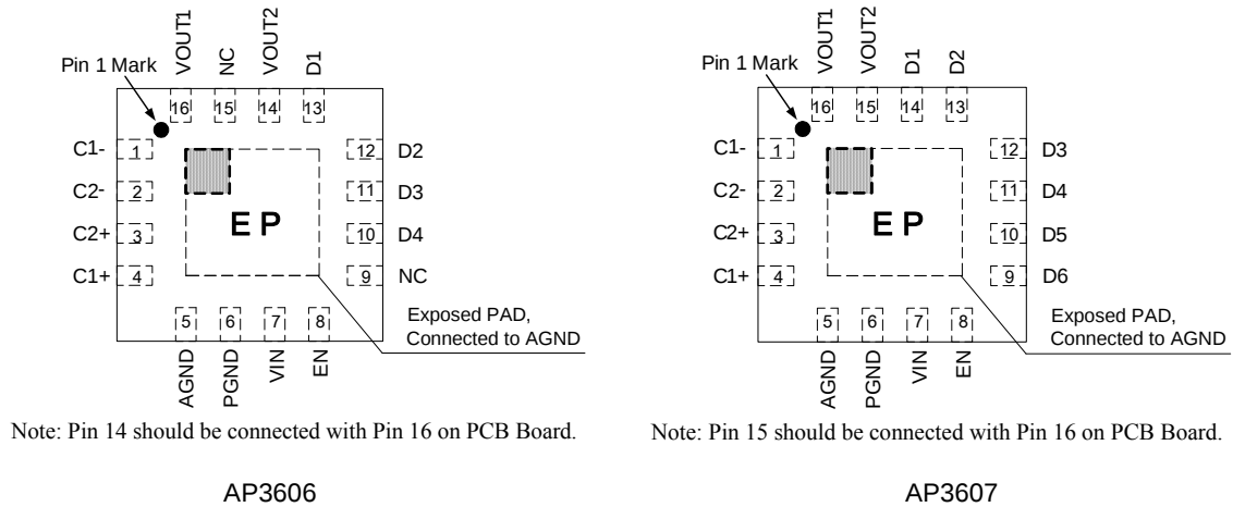
Figure 2. Pin Configuration of AP3606/AP3607 (Top View)
