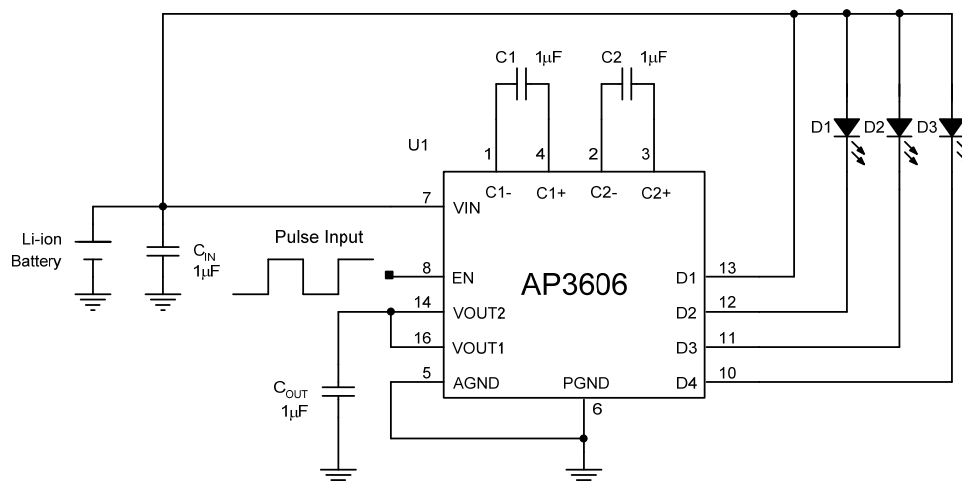
3 WLEDs
