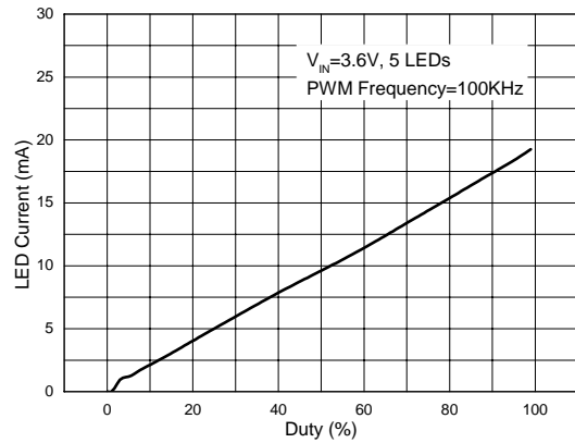
Figure 17. LED Current vs. Duty
