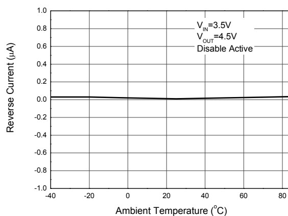
Figure 11. Reverse Current vs. Ambient Temperature
