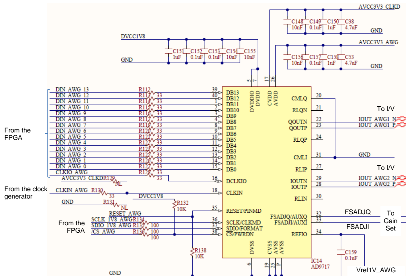
Figure 15. DAC
