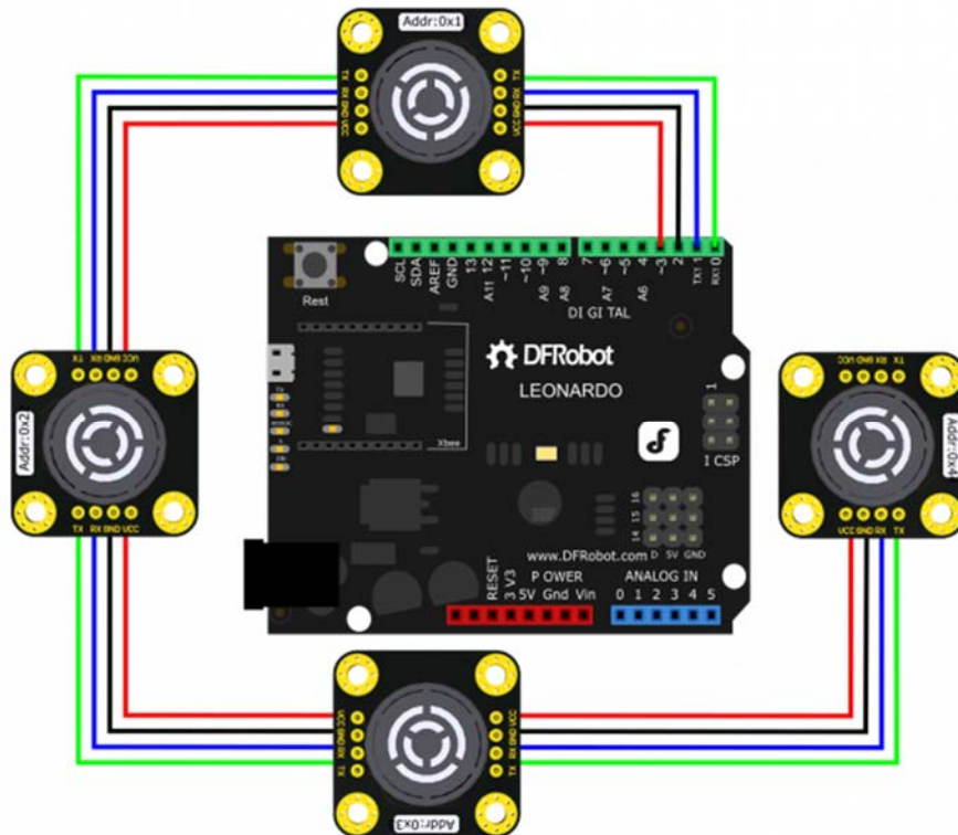
Read Distance Value via Arduino (Cascade)
