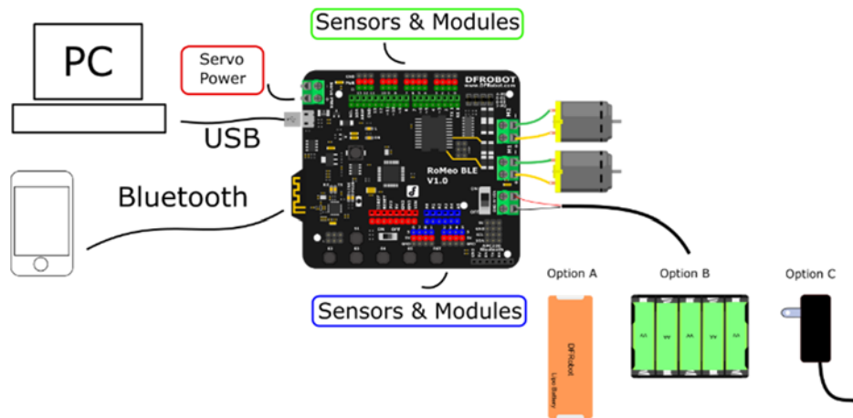
Romeo BLE with Motors connection
