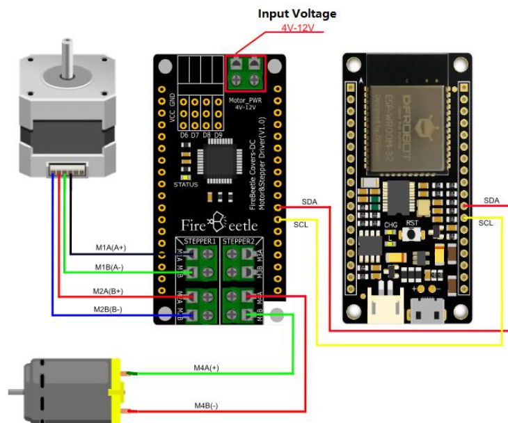
DC Motor & Stepper Drive Wiring Diagram
