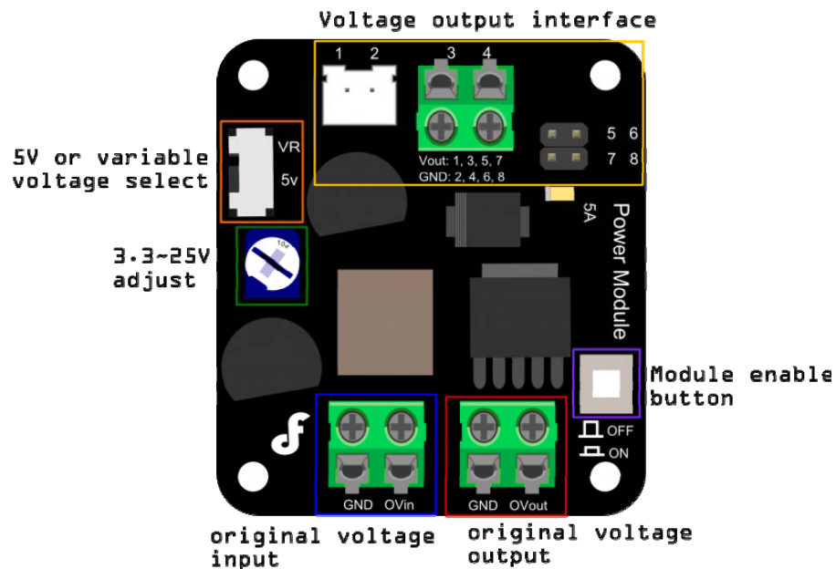
Power Module diagram
