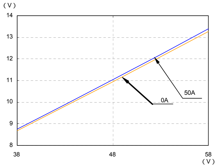
Figure 4: Output voltage regulation vs input Voltage, for minimum current and maximum current
