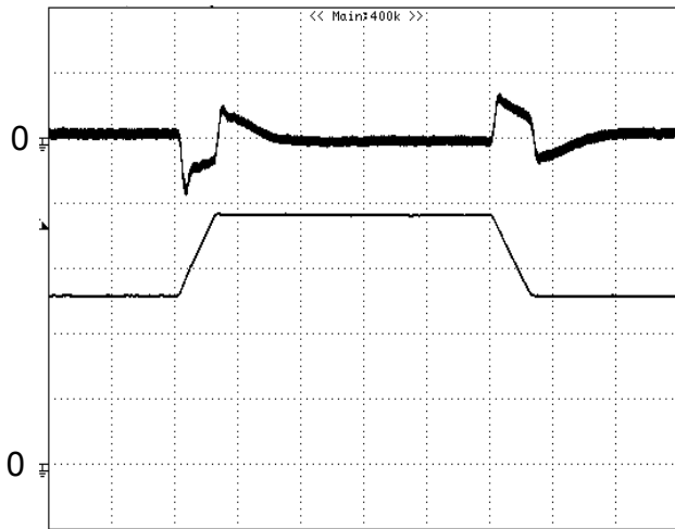
Figure 9: Output voltage response to step-change in load current (50%-75%-50% of I_{o, max} ; di/dt = 0.1A/\mu s ). Load cap: 10\mu F , tantalum capacitor and 1\mu F ceramic capacitor. Top Trace: V_{out} (100mV/div, 200us/div), Bottom Trace: I_{out} (10A/div). Scope measurement should be made using a BNC cable (length shorter than 20 inches). Position the load between 51 mm to 76 mm (2 inches to 3 inches) from the module.
