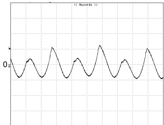
Figure 10: Output voltage response to step-change in load current (50%-75%-50% of I_{o, max} ; di/dt = 1A/\mu s ). Load cap: 10\mu F , tantalum capacitor and 1\mu F ceramic capacitor. Top Trace: V_{out} (500mV/div, 200us/div), Bottom Trace: I_{out} (10A/div). Scope measurement should be made using a BNC cable (length shorter than 20 inches). Position the load between 51 mm to 76 mm (2 inches to 3 inches) from the module.
