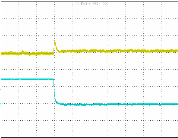
Figure 19: Typical transient response to step load change at 2.5A/\mu S from 50% to 0% of I_o , max at 5Vin, 0.6Vout (200uS/div) ( C_{out} = 47\mu F ceramic). top trace: Vout, 0.1V/div; bottom trace: Iout, 2A/div.
