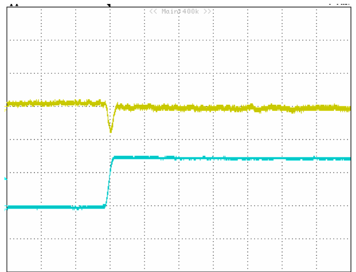
Figure 22: Typical transient response to step load change at 2.5A/\mu S from 0% to 50% of I_o , max at 5Vin, 1.2Vout (200uS/div) ( C_{out} = 47\mu F ceramic). top trace: Vout, 0.1V/div; bottom trace: Iout, 2A/div.
