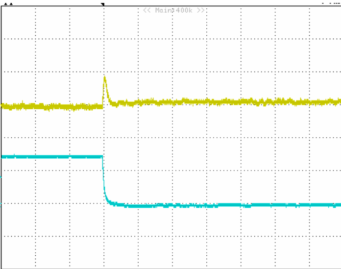
Figure 21: Typical transient response to step load change at 2.5A/\mu S from 50% to 0% of I_o , max at 5Vin, 1.2Vout (200uS/div) ( C_{out} = 47\mu F ceramic). top trace: Vout, 0.1V/div; bottom trace: Iout, 2A/div.
