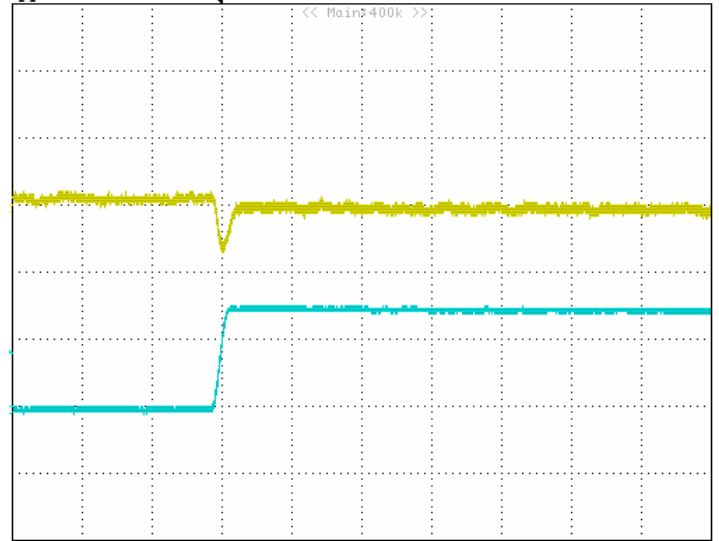
Figure 20: Typical transient response to step load change at 2.5A/\mu S from 0% to 50% of I_o , max at 5Vin, 0.6Vout (200uS/div) ( C_{out} = 47\mu F ceramic). top trace: Vout, 0.1V/div; bottom trace: Iout, 2A/div.
