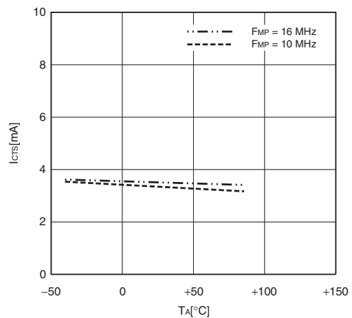
I_{CTS} - T_A V_{CC} = 3.0 \text{ V} , F_{MP} = 10, 16 \text{ MHz} (divided by 2) Time-base timer mode with the external clock operating
