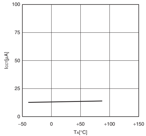
I_{CCT} - T_A V_{CC} = 3.0 \text{ V} , F_{MPL} = 16 \text{ kHz} (divided by 2) Watch mode with the external clock operating
