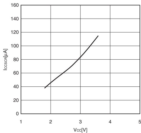
I_{CCSCR} - V_{CC} T_A = +25^\circ\text{C} , F_{MPL} = 50 \text{ kHz} (divided by 2) Substop mode with the sub-CR clock operating
