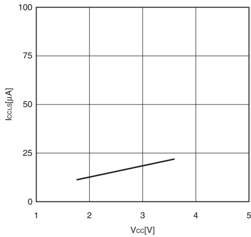
I_{CCLS} - V_{CC} T_A = +25^\circ\text{C} , F_{MPL} = 16 \text{ kHz} (divided by 2) Subsleep mode with the external clock operating
