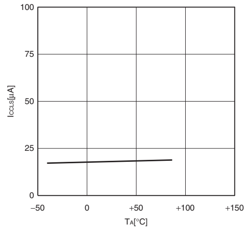
I_{CCLS} - T_A V_{CC} = 3.0 \text{ V} , F_{MPL} = 16 \text{ kHz} (divided by 2) Subsleep mode with the external clock operating
