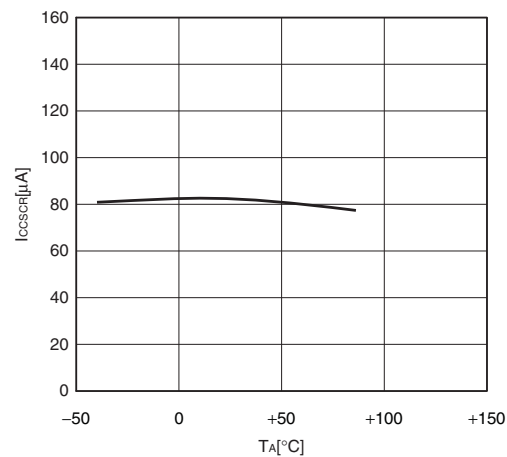
I_{CCSCR} - T_A V_{CC} = 3.0 \text{ V} , F_{MPL} = 50 \text{ kHz} (divided by 2) Substop mode with the sub-CR clock operating
