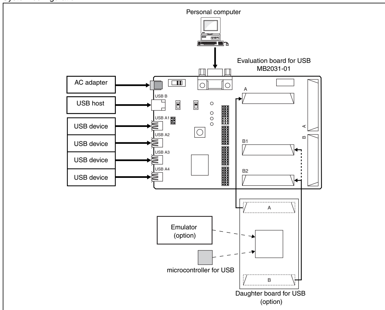
System configuration
