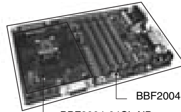
BBF2004-64CL-NB (NQPAC Type daughter board LQFP-64)
