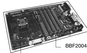
BBF2004-64CL-NB (NQPACK Type daughter board LQFP-64)
