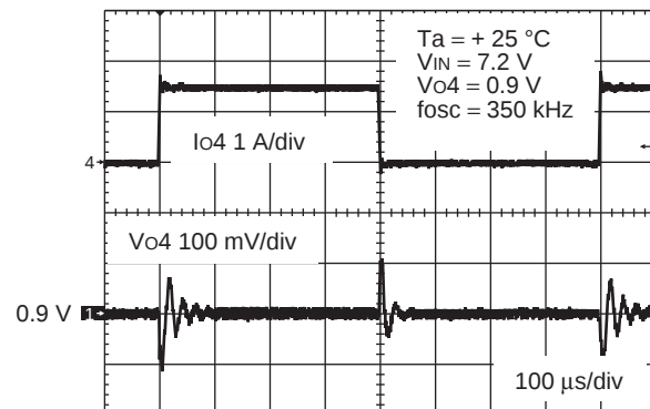
CH4 (fosc = 350 kHz, Vo4 = 0.9 V)
