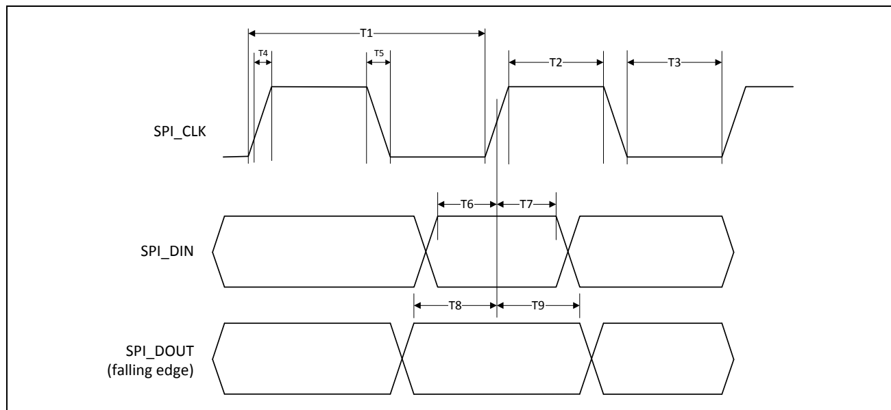
Figure 46: gSPI Timing
