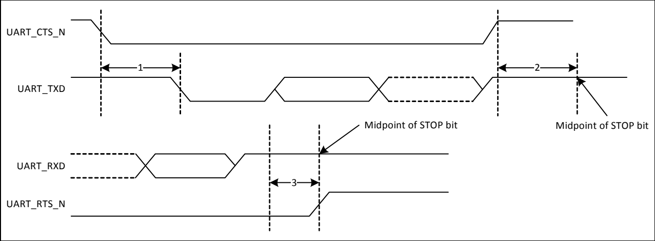
Figure 18: UART Timing
