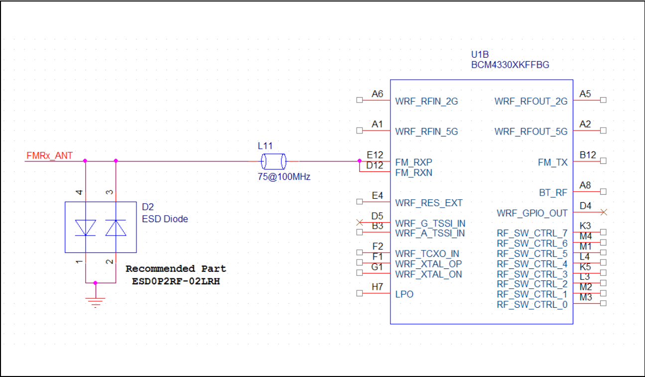
Figure 42: FM Receiver Circuit
