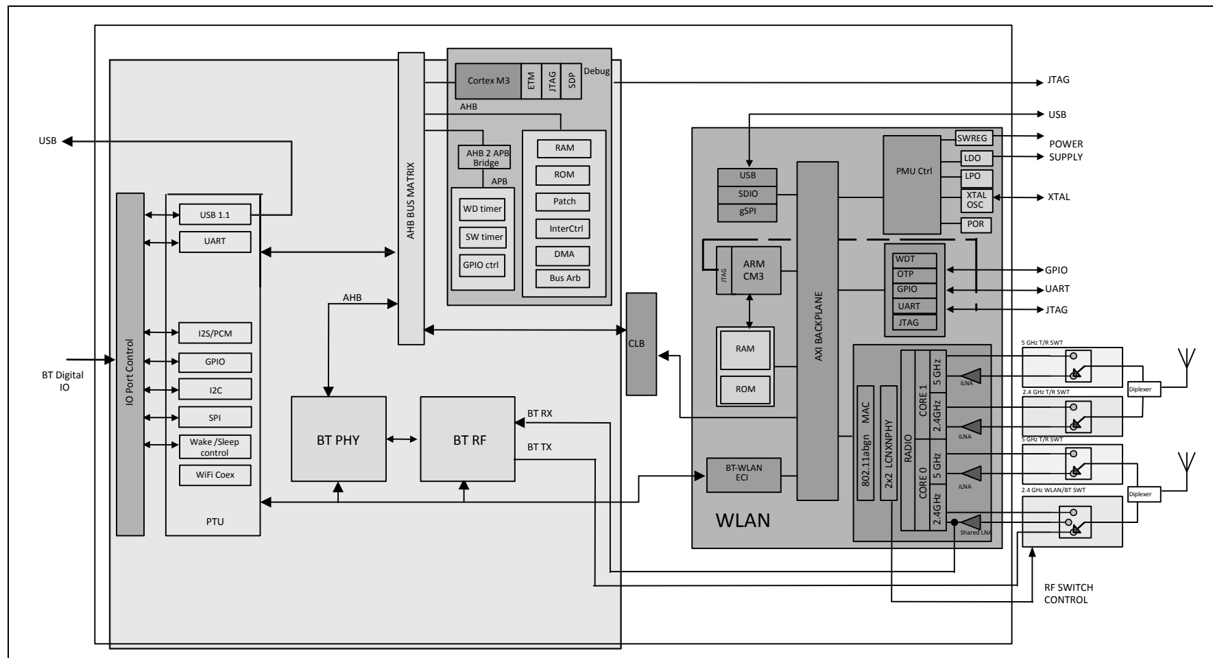
Figure 2: BCM43242 Block Diagram
