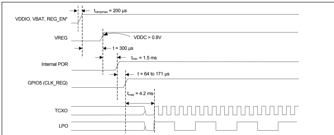
Figure 11. Startup Timing from Power-on Reset
