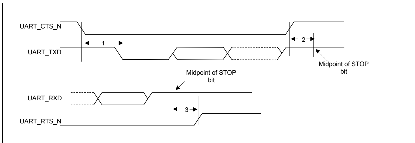
Figure 12. UART Timing
