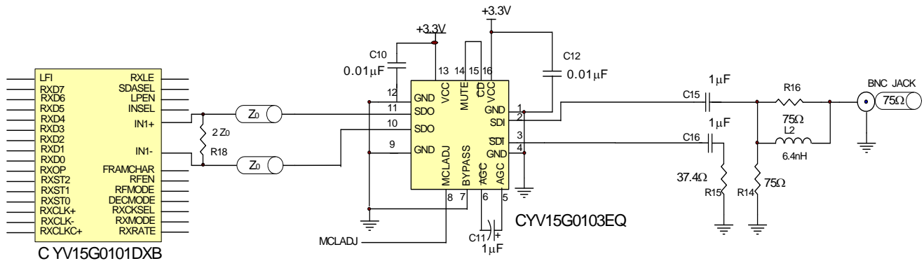
Figure 3. Interfacing CYV15G0103EQ to the HOTLink II SerDes
