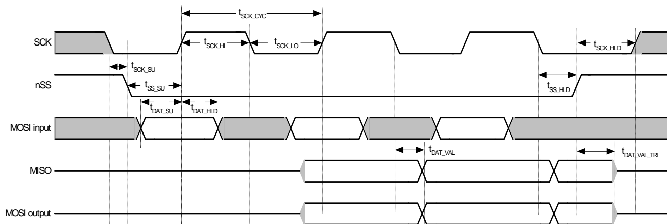
Figure 11. SPI Timing
