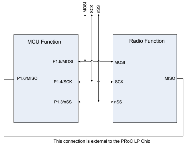
Figure 7. 4-Wire SPI Mode
