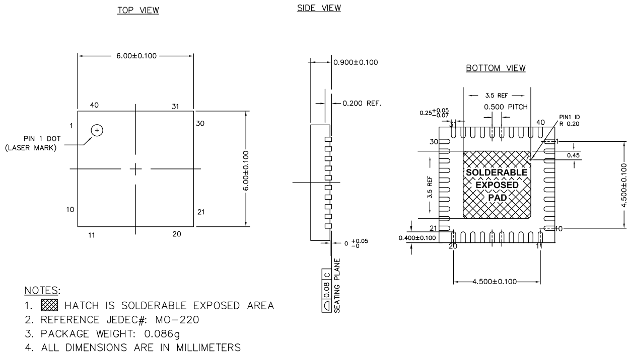
Figure 26. 40-pin QFN (6 × 6 × 1.0 mm) LT40B 3.50 × 3.50 E-Pad (Sawn) Package Outline
