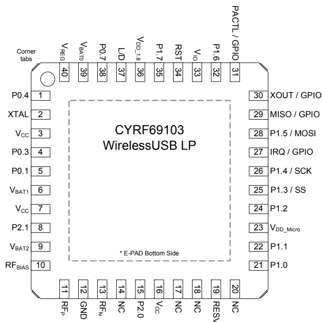
Figure 1. Pin Diagram
