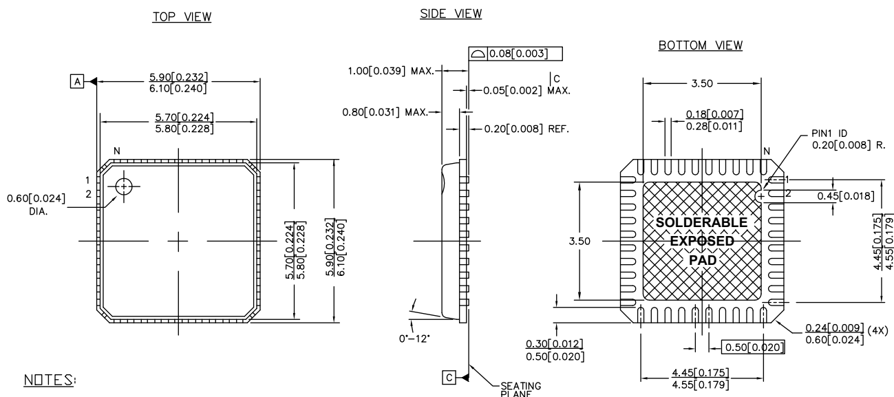
Figure 25. 40-pin QFN (6 × 6 × 1.0 mm) LF40A/LY40A 3.50 × 3.50 E-Pad (Sbcon Punch Type Package) Package Outline
