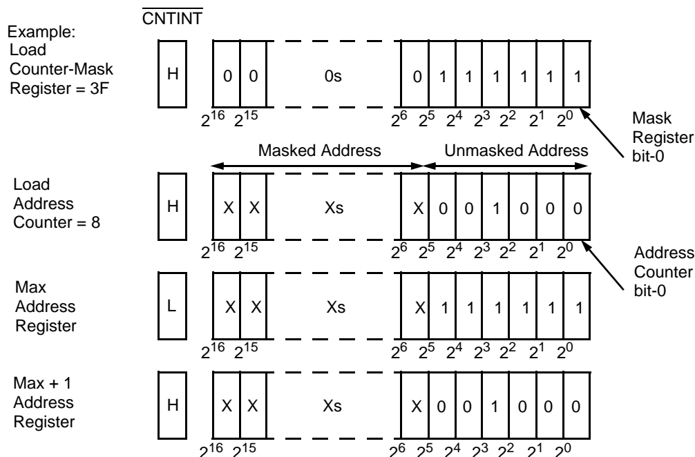
Figure 2. Programmable Counter-Mask Register Operation [31, 32]
