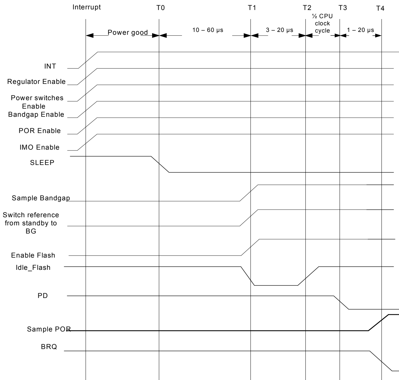
Figure 10-2. Wakeup Sequence for the Device 123
