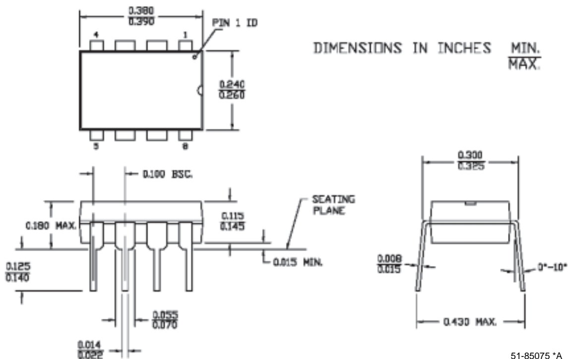
Figure 2-1. 8-Lead (300-Mil) PDIP
