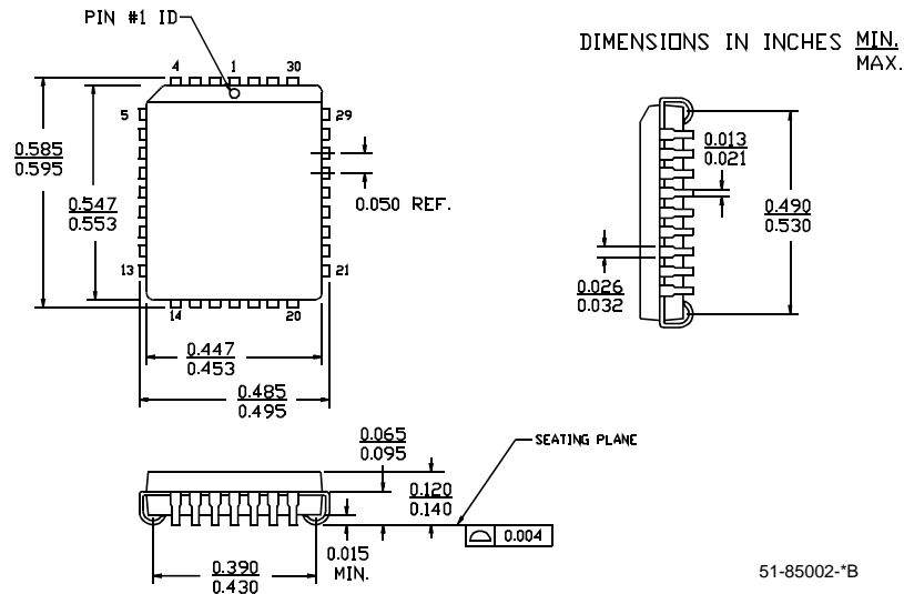
32-Lead Plastic Leaded Chip Carrier J65
