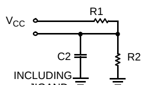
(b) output load for t HZOE , t HZCE , t HZWE
