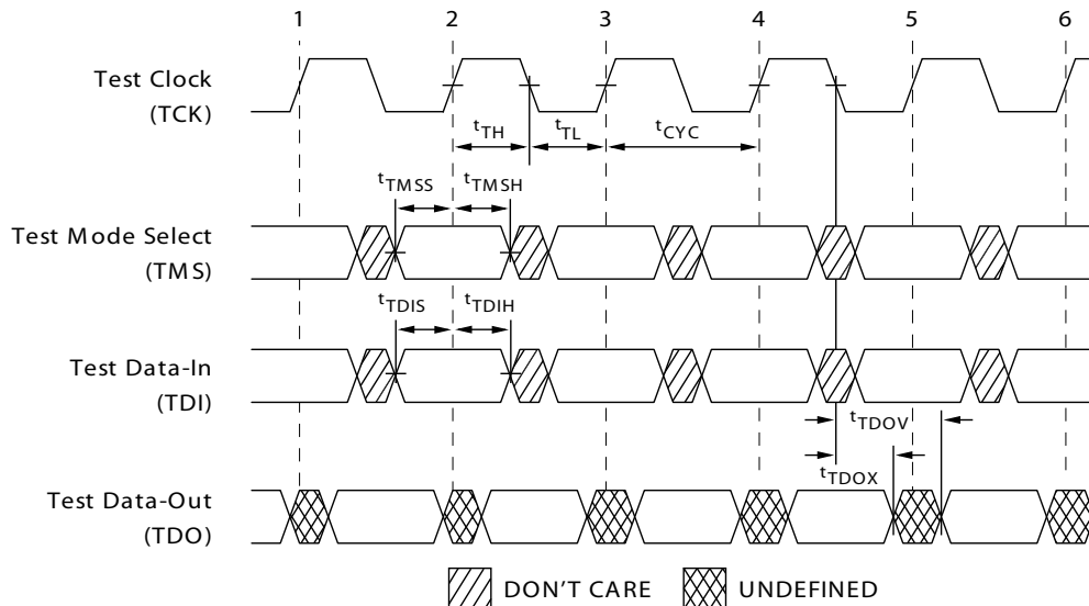
Figure 4. TAP Timing
