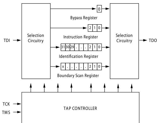
Figure 4. TAP Controller Block Diagram
