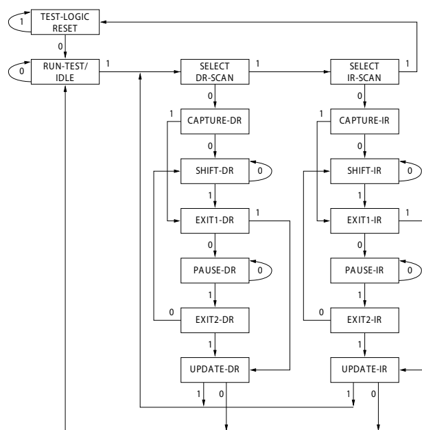
Figure 3. TAP Controller State Diagram
