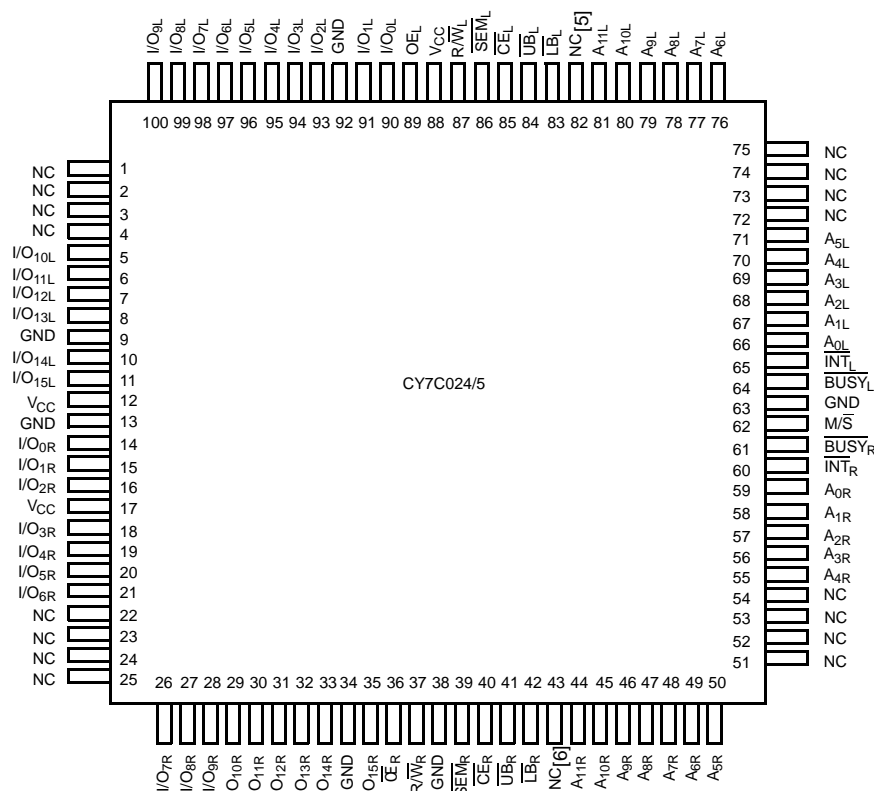
Figure 2. 100-Pin TQFP (Top View)
