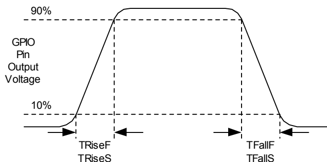
Figure 12. GPIO Timing Diagram
