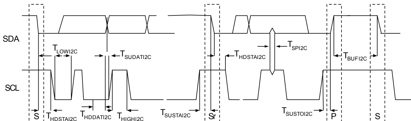
Figure 15. Definition for Timing for Fast/Standard Mode on the I 2 C Bus
