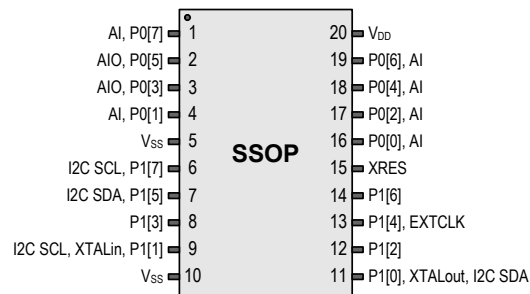
Figure 3. CY8C24223A 20-Pin PSoC Device
