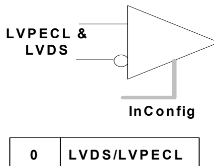
Figure 7. LVDS/LVPECL [6]
