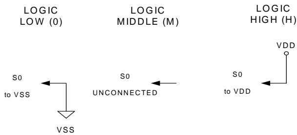
Figure 1. 3-Level Logic
