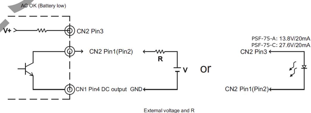
Internal Circuit of AC OK and Battery Low
