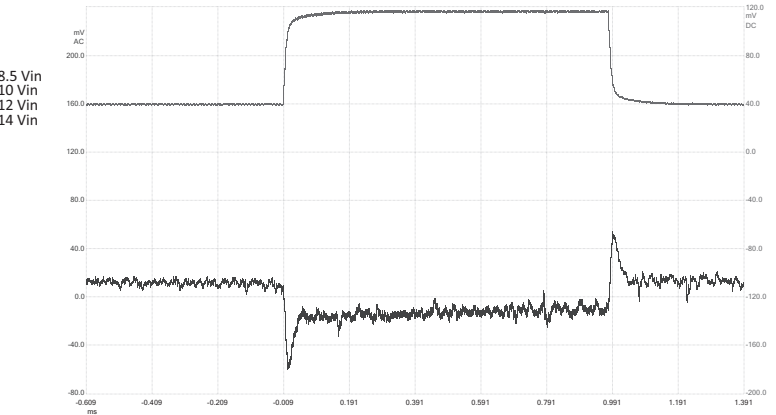
Top Trace: Load Current Bottom Trace: Output Voltage (40 mV / div) Current step-change (6.25-18.75-6.25 A) Time Scale: (200 \mu\text{s} / div) Slew Rate: (1A/ \mu\text{s} )
