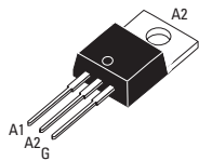
T0-220AB Non-Isolated (CTB12)
