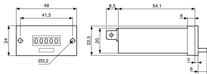
24 x 48 - 5 decades 99 766 92●
