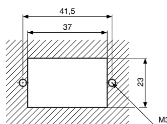
Panel cut-out 99 766 9●●
