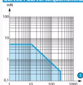
Curves : Curve: torque/nominal speed 827470
