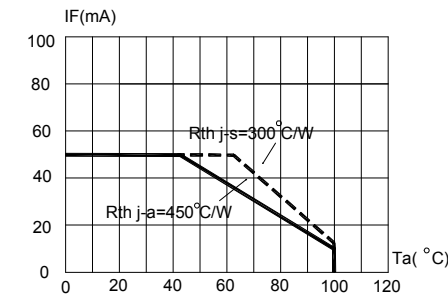
FIG.4a RED MAXIMUM FORWARD DCCURRENT VS AMBIENT TEMPERATURE (Tjmax=110°C)
