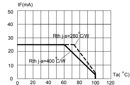
FIG.4b GREEN MAXIMUM FORWARD DCCURRENT VS AMBIENT TEMPERATURE (Tjmax=110°C)
