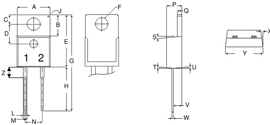
Package TO-220-2
