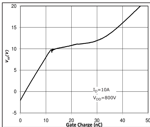
Fig 8. Typical Gate Charge Characteristics @ 25^\circ\text{C}
